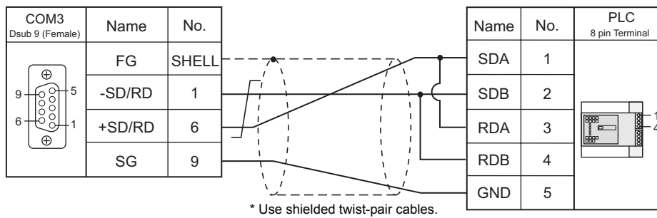
Wiring diagram 2 - COM3
