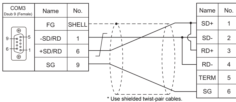
Wiring diagram 2 - COM3
