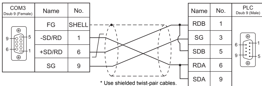
Wiring diagram 4 - COM3
