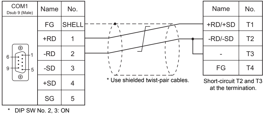
Wiring diagram 1 - COM1
