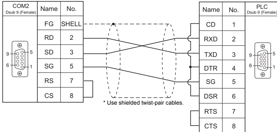
Wiring diagram 1 - COM2
