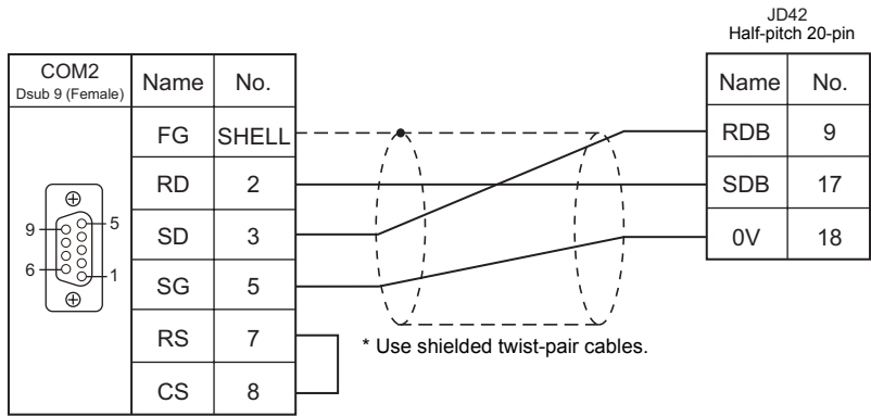
Wiring diagram 1 - COM2
