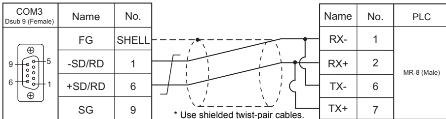
Wiring diagram 3 - COM3
