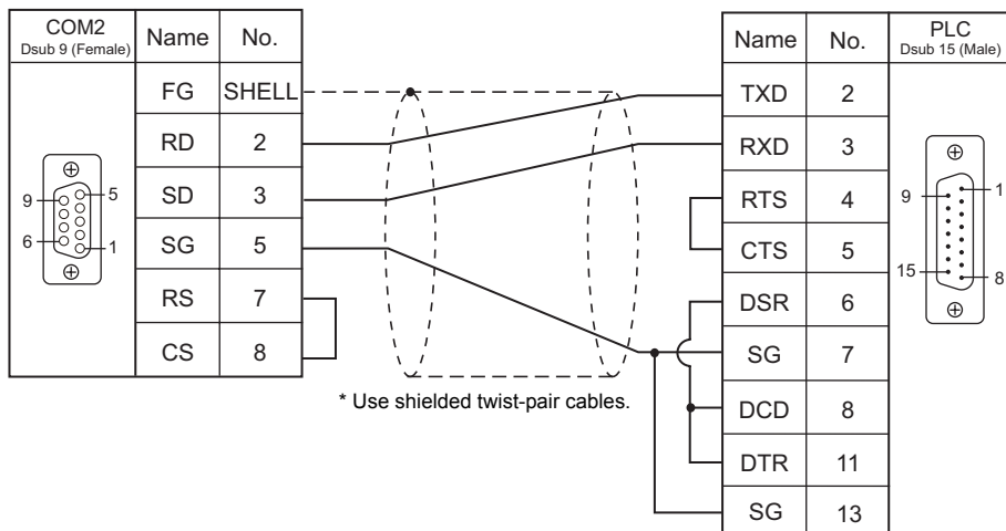
Wiring diagram 3 - COM2
