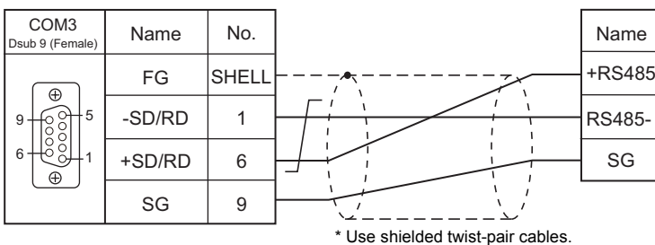
Wiring diagram 1 - COM3
