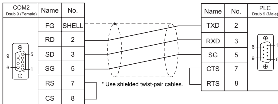
Wiring diagram 4 - COM2
