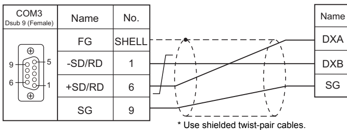
Wiring diagram 4 - COM3
