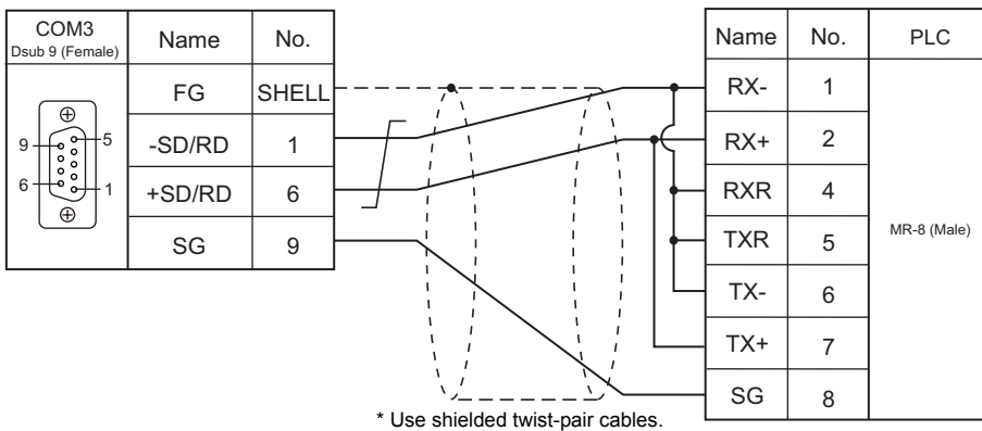
Wiring diagram 4 - COM3
