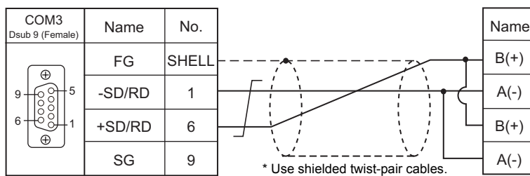
Wiring diagram 2 - COM3
