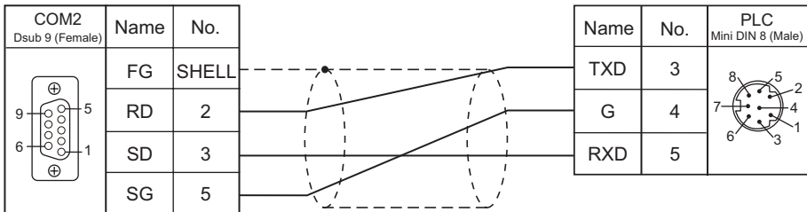
Wiring diagram 3 - COM2
