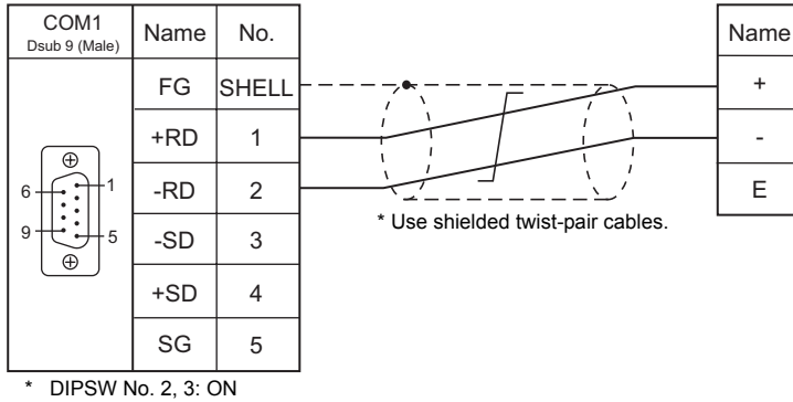
Eco-POWER METER connected at the terminal (except for KW4M)
