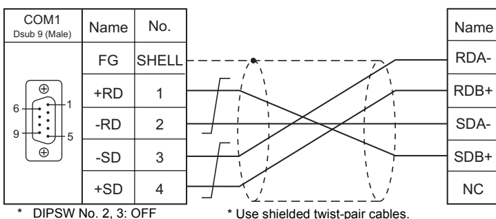
Wiring diagram 4 - COM1
