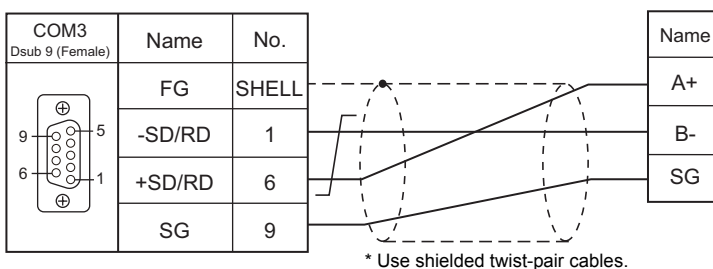
Wiring diagram 5 - COM3
