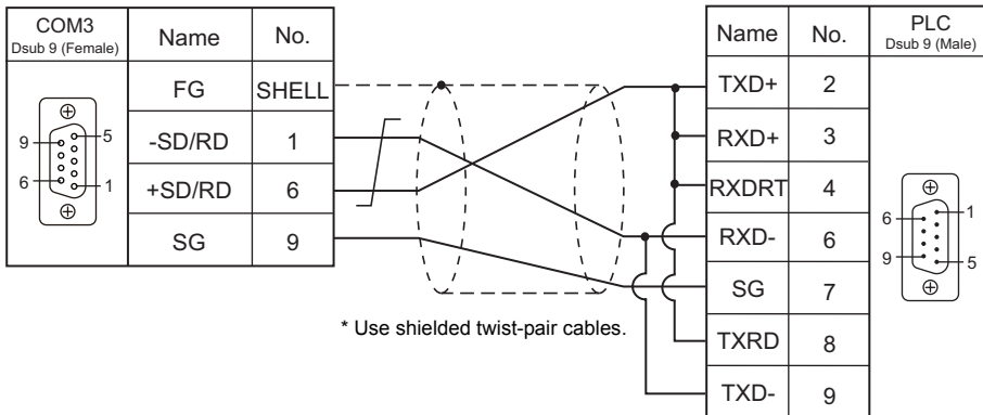
Wiring diagram 3 - COM3
