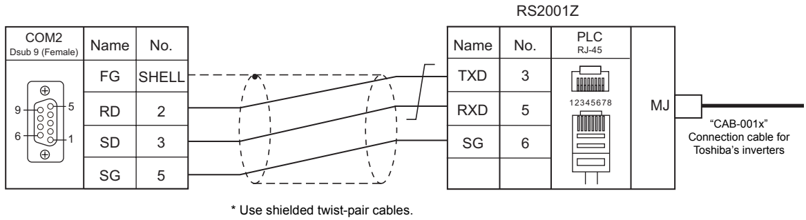
Wiring diagram 1 - COM2
