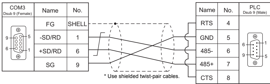
Wiring diagram 2 - COM3
