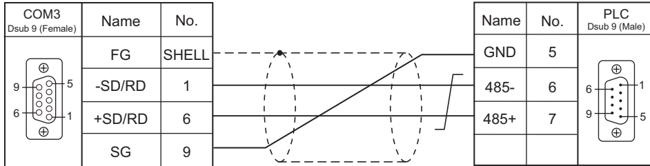
Wiring diagram 1 - COM3
