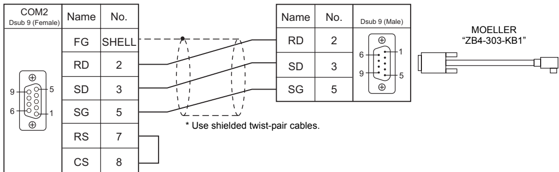
Wiring diagram 2 - COM2
