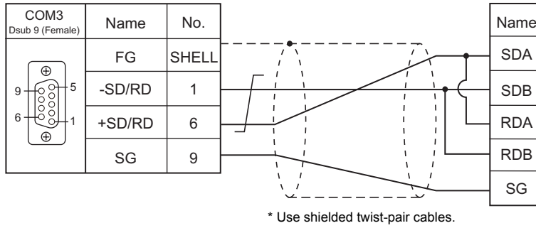
Wiring diagram 1 - COM3
