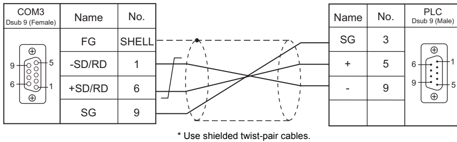
Wiring diagram 3 - COM3
