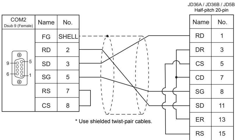
Wiring diagram 2 - COM2
