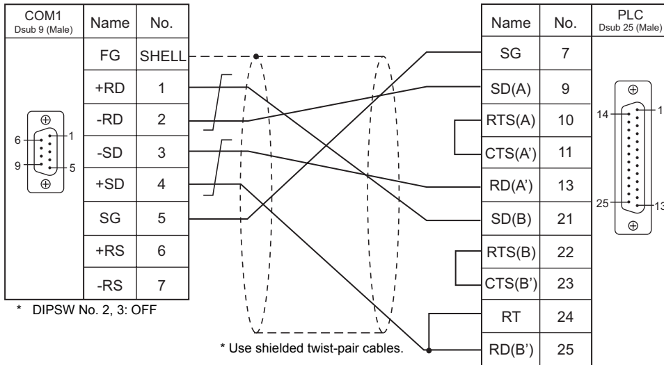
Wiring diagram 2 - COM1
