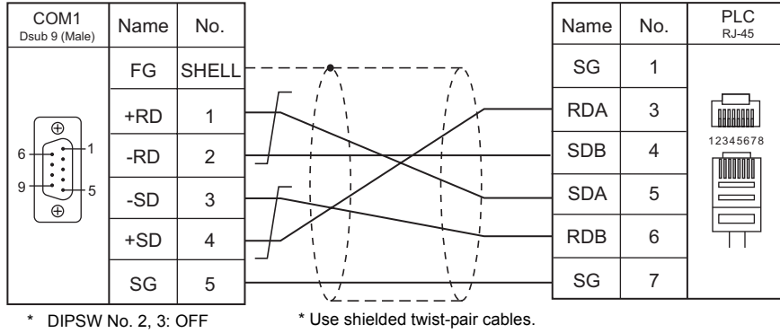
Wiring diagram 1 - COM1
