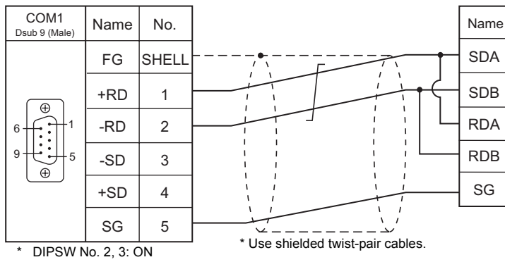
Wiring diagram 2 - COM1
