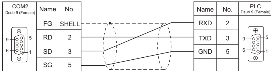
Wiring diagram 1 - COM2
