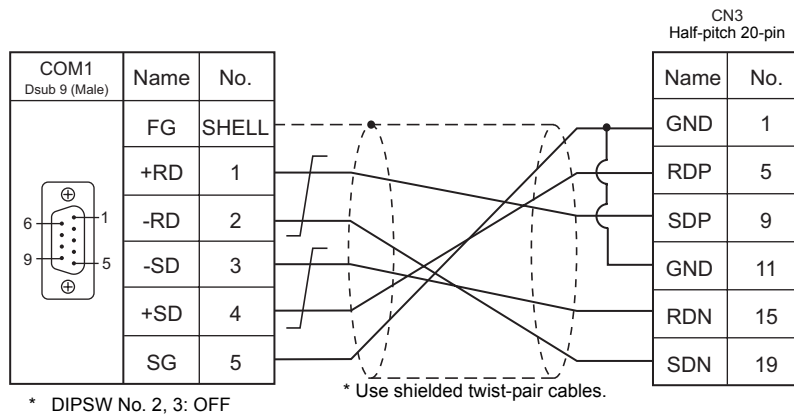
Wiring diagram 2 - COM1
