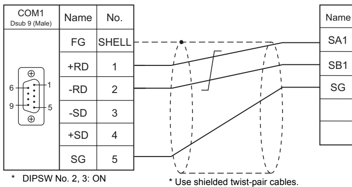
Wiring diagram 3 - COM1
