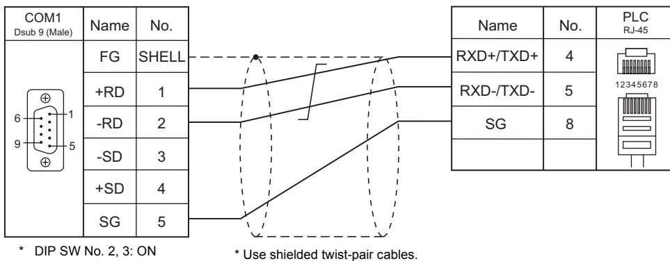
Wiring diagram 3 - COM1
