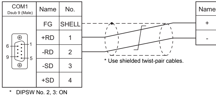
Wiring diagram 1 - COM1
