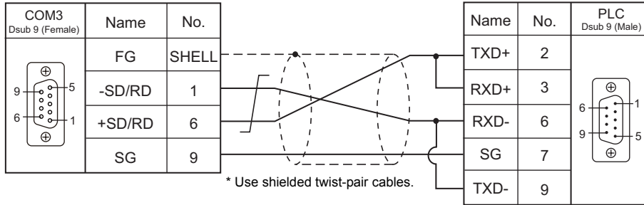
Wiring diagram 1 - COM3
