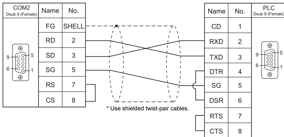
Wiring diagram 3 - COM2
