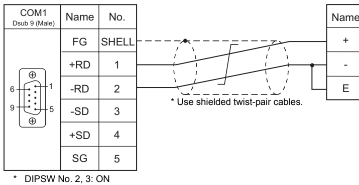
Eco-POWER METER connected at the terminal (except for KW4M)
