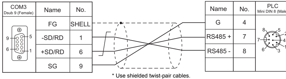
Wiring diagram 2 - COM3
