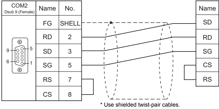
Wiring diagram 1 - COM2
