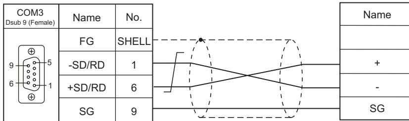
Wiring diagram 1 - COM3
