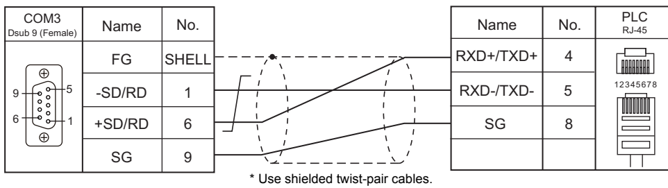
Wiring diagram 3 - COM3
