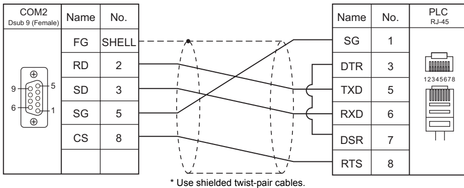
Wiring diagram 3 - COM2
