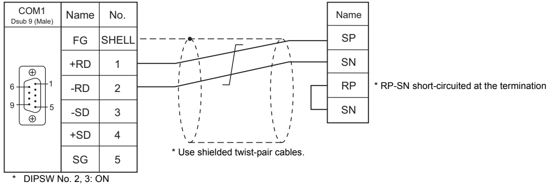
Wiring diagram 1 - COM1
