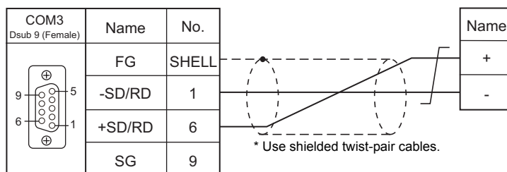
Wiring diagram 1 - COM3
