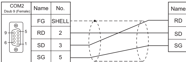
Wiring diagram 2 - COM2
