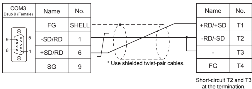
Wiring diagram 1 - COM3
