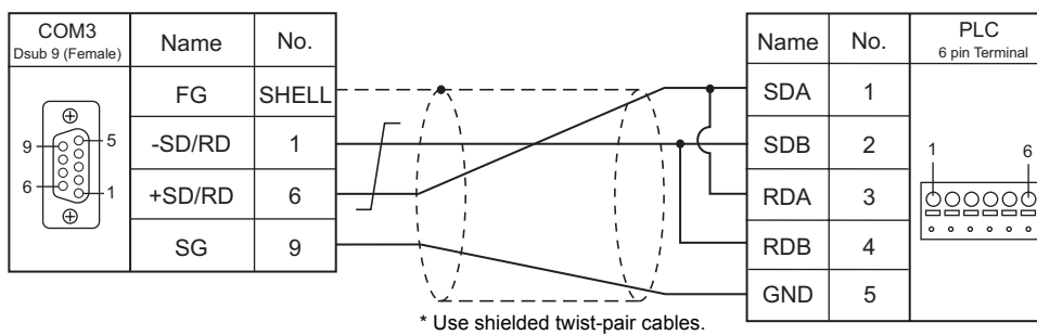
Wiring diagram 4 - COM3
