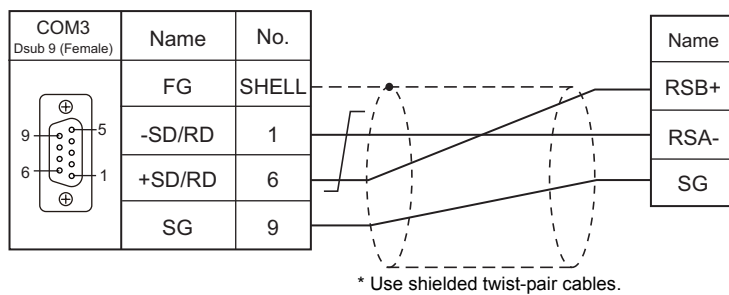
Wiring diagram 2 - COM3
