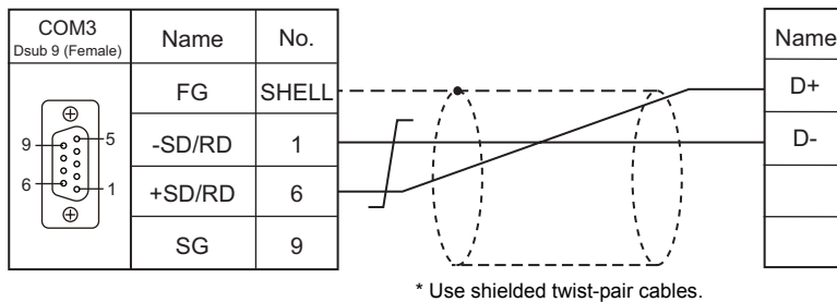
Wiring diagram 2 - COM3
