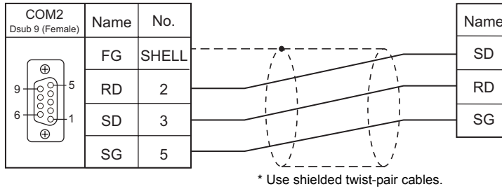
Wiring diagram 1 - COM2
