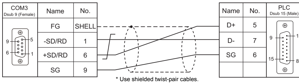
Wiring diagram 1 - COM3
