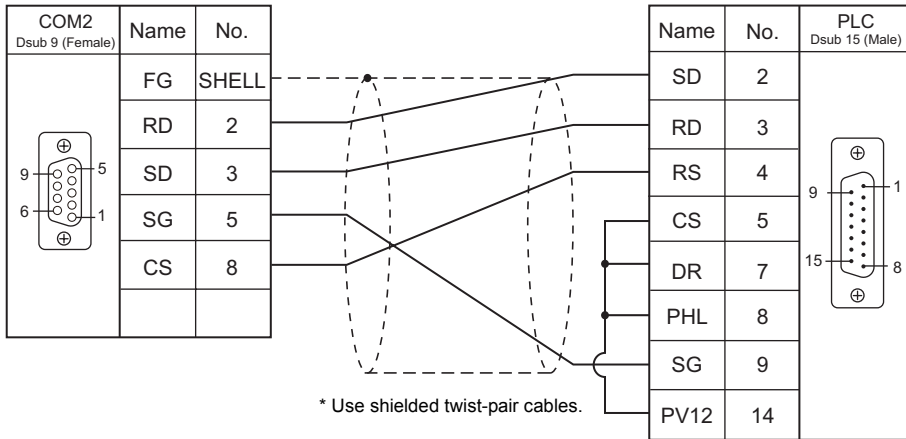
Wiring diagram 2 - COM2
