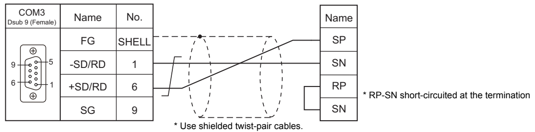
Wiring diagram 1 - COM3
