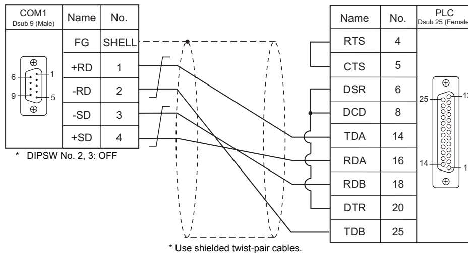
Wiring diagram 2 - COM1
