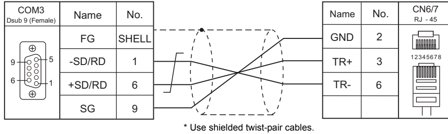
Wiring diagram 1 - COM3
