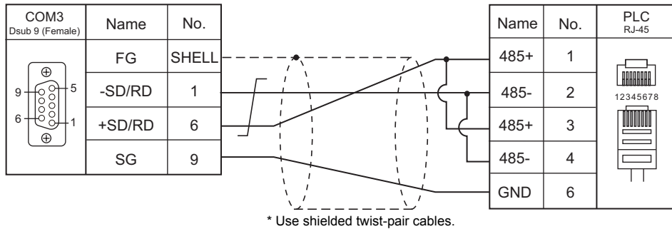
Wiring diagram 3 - COM3
