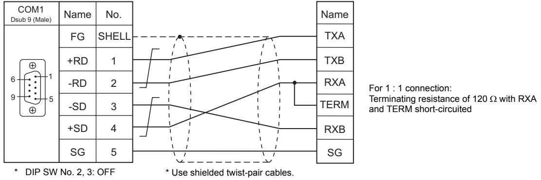
Wiring diagram 1 - COM1
