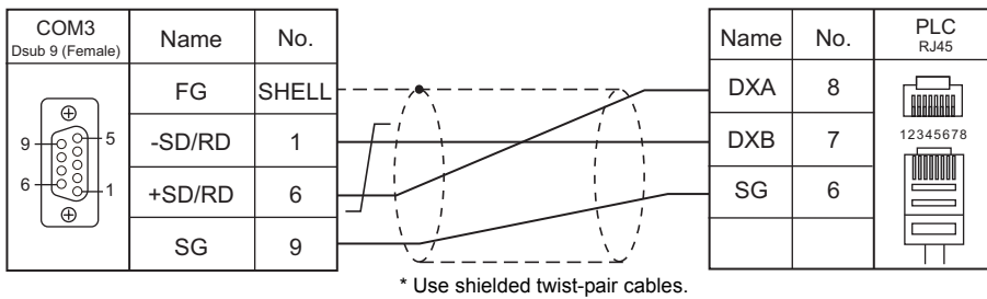
Wiring diagram 3 - COM3
