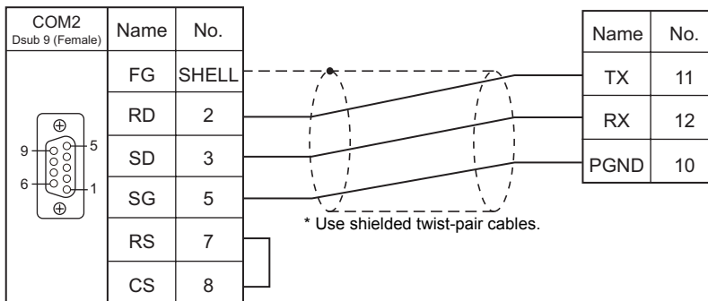
Wiring diagram 2 - COM2
