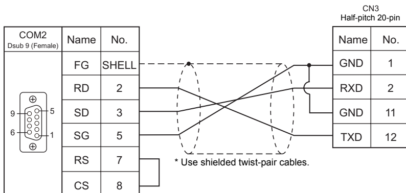
Wiring diagram 1 - COM2
