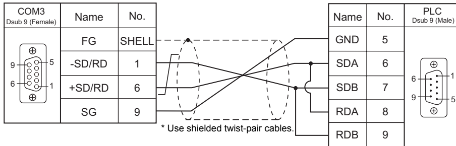
Wiring diagram 1 - COM3
