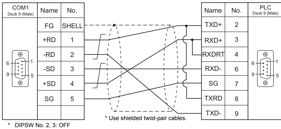
Wiring diagram 3 - COM1
