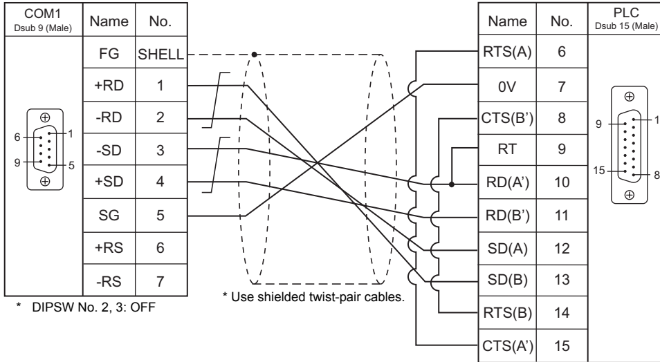
Wiring diagram 1 - COM1
