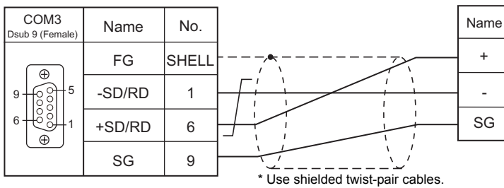
Wiring diagram 3 - COM3
