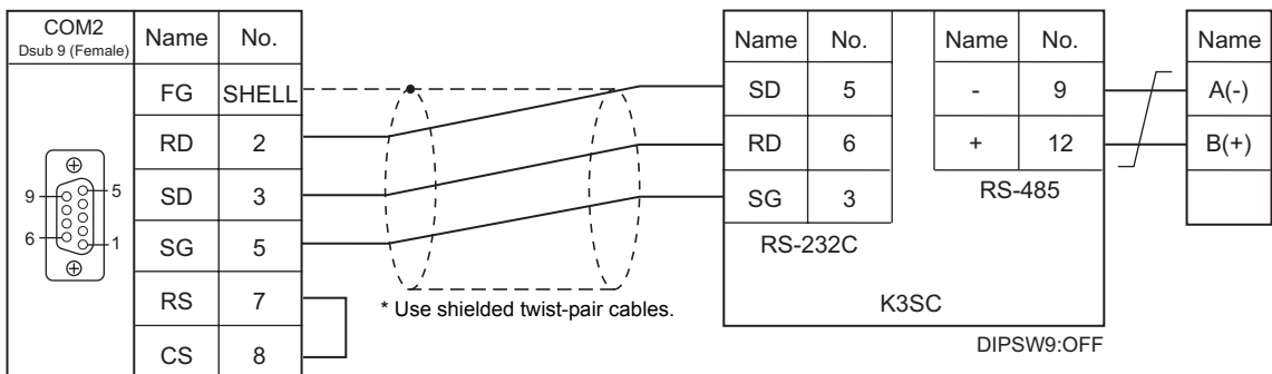
Wiring diagram 4 - COM2
