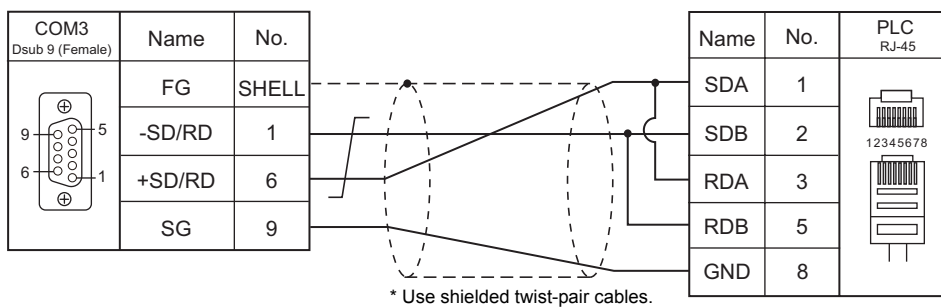
Wiring diagram 3 - COM3
