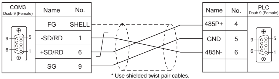
Wiring diagram 4 - COM3
