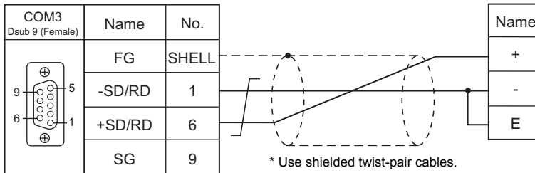
Eco-POWER METER connected at the terminal (except for KW4M)
