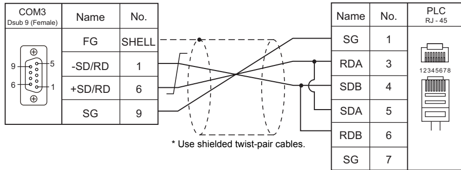
Wiring diagram 1 - COM3
