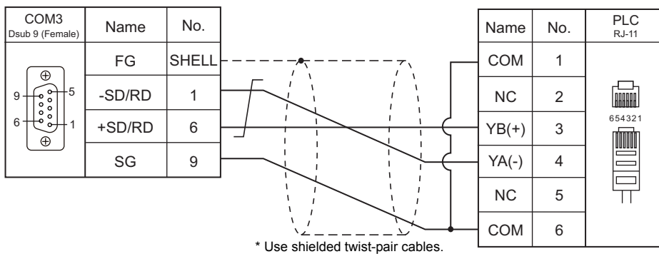
Wiring diagram 2 - COM3
