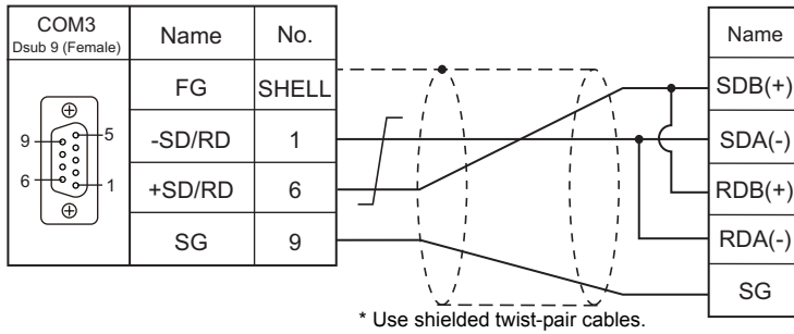
Wiring diagram 1 - COM3
