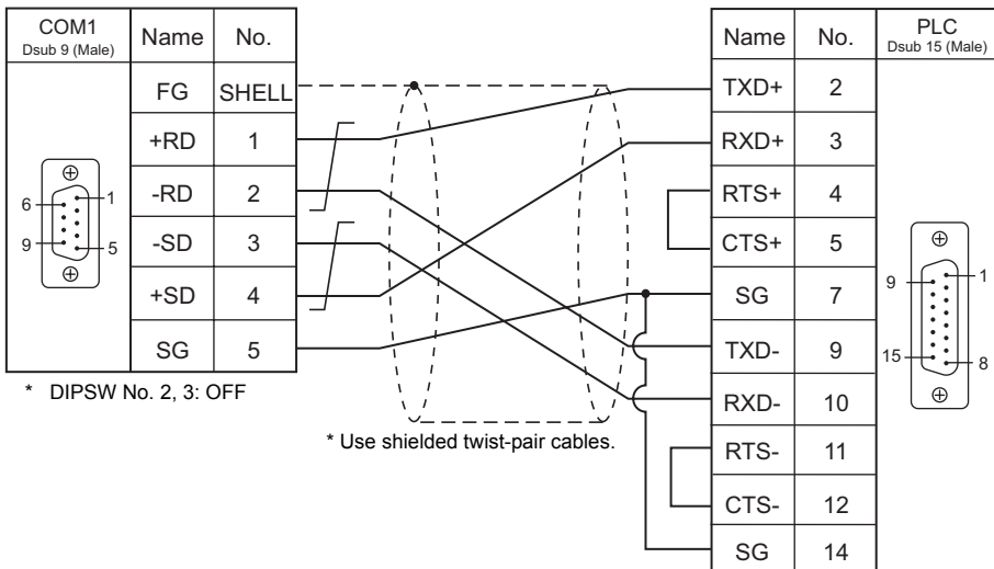
Wiring diagram 2 - COM1
