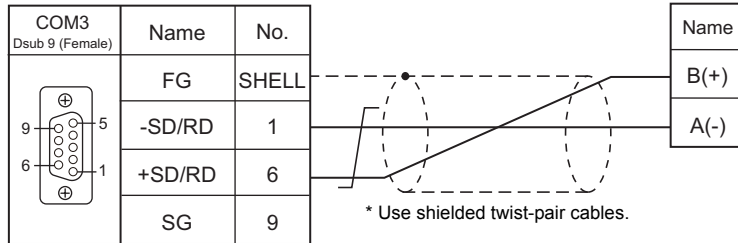
Wiring diagram 1 - COM3
